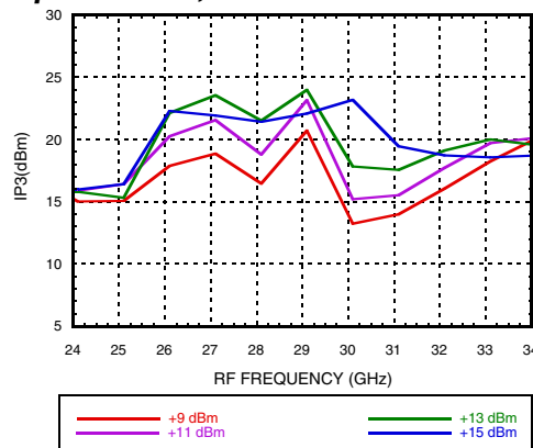
Input IP3 vs. LO Power Upconverter, LO= 11 GHz
