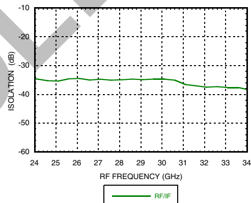
Isolation RF/IF
