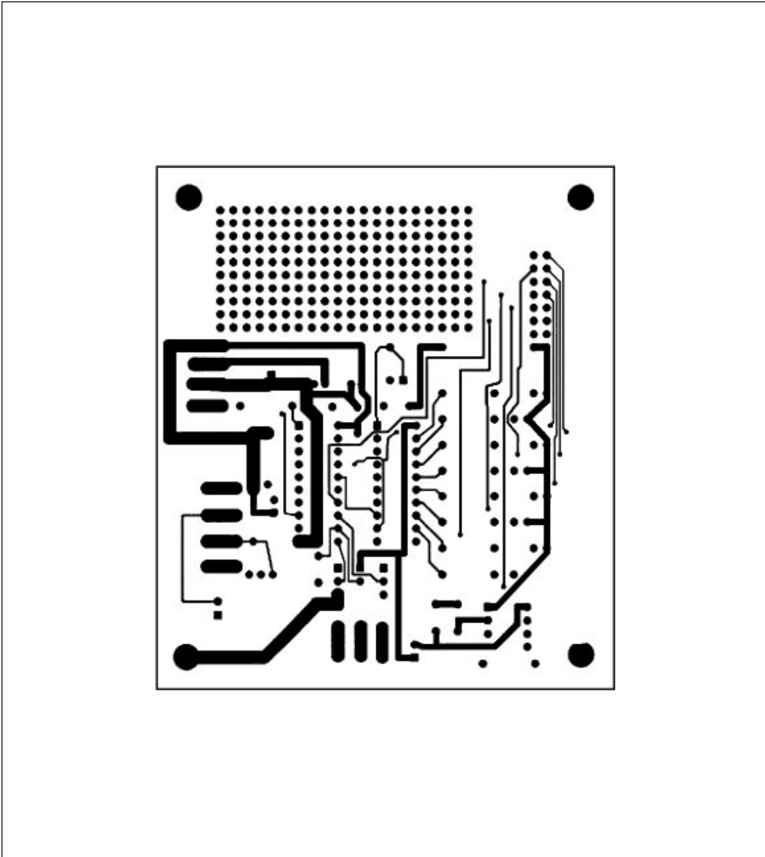
Figure 3. MAX152 EV Kit Solder-Side Layout (Mirror Image)
