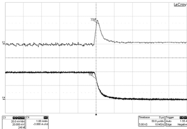
Figure 9. Load transient 2.0 A to 0.2 A, with V_{OUT} = 3.3\text{ V} and V_{IN} = 13.2\text{ V}
