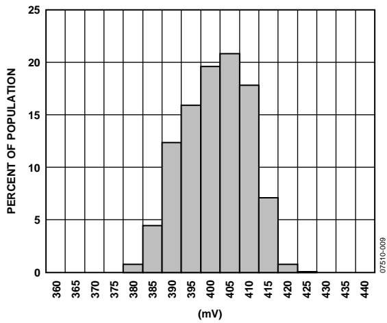
Figure 13. ADXL001-70, Self-Test Delta
