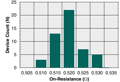
Typical On-Resistance Distribution (N=50, I_F=1\text{mA} , I_L=400\text{mA} )
