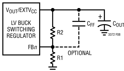
Figure 8. Feedback Components
