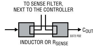
Figure 2. Sense Lines Placement with Inductor or Sense Resistor
