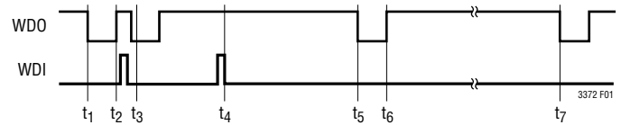
Figure 1. WDO Timing Parameters
