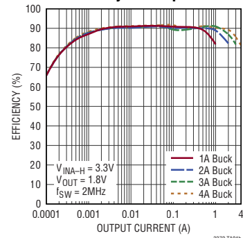
Low Voltage Buck Regulator Configurations
