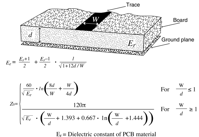
Figure 63: Microstrip Formulas
