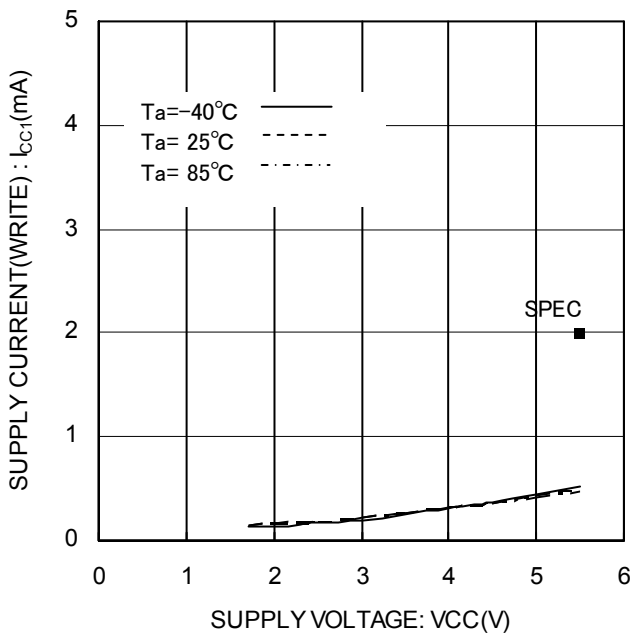
Figure 14. Supply current (WRITE) I_{cc1}(\text{WRITE}, f_{sk}=3\text{MHz})
