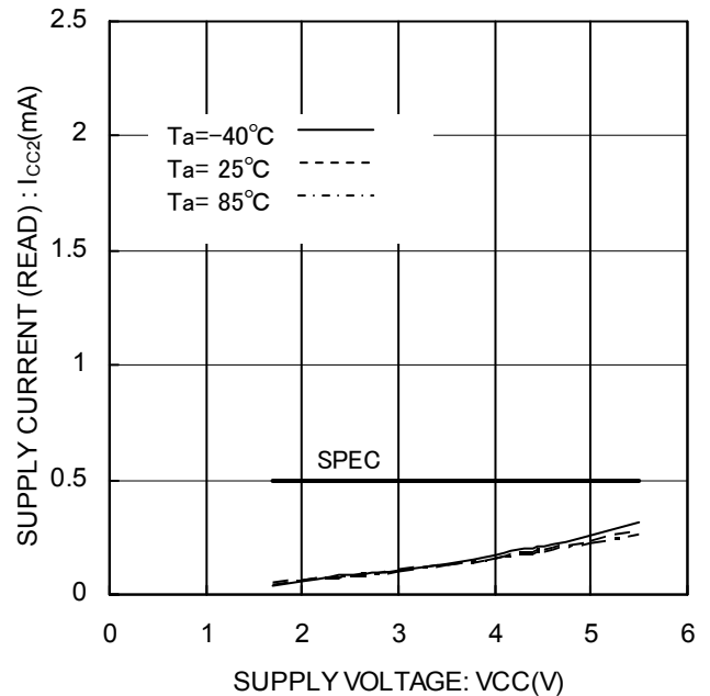
Figure 15. Supply current (READ) I_{cc2}(\text{READ}, f_{sk}=1\text{MHz})
