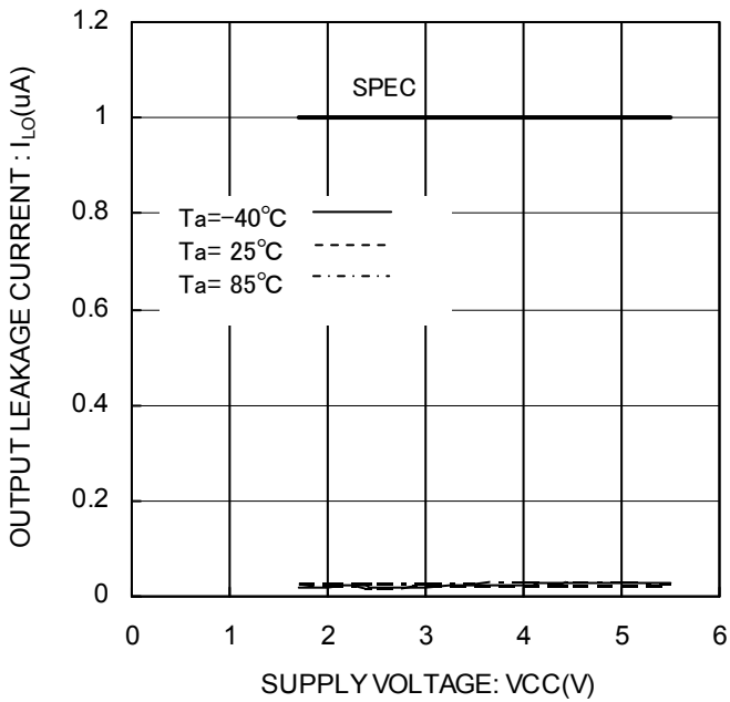
Figure 12. Output leakage current I_{Lo}(\text{DO})
