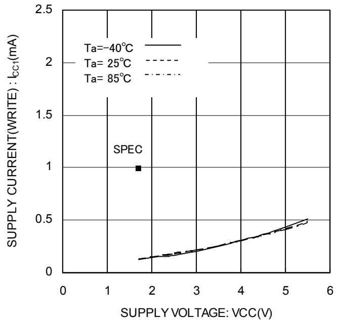
Figure 13. Supply current (WRITE ) I_{cc1}(\text{WRITE}, f_{sk}=1\text{MHz})
