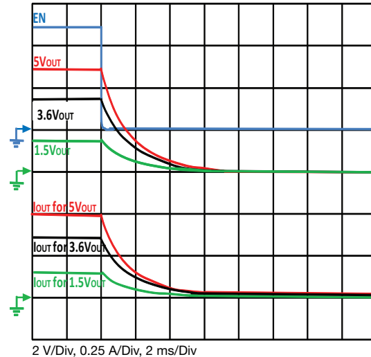
Fig. 26 - Typical Fall Time C_{OUT} = 200 \mu\text{F} , C_{IN} = 4.7 \mu\text{F} , R_{OUT} = 10 \Omega
