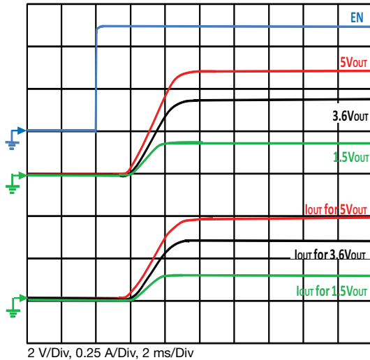
Fig. 25 - Typical Turn-On Delay, Rise Time C_{OUT} = 200 \mu\text{F} , C_{IN} = 4.7 \mu\text{F} , R_{OUT} = 10 \Omega
