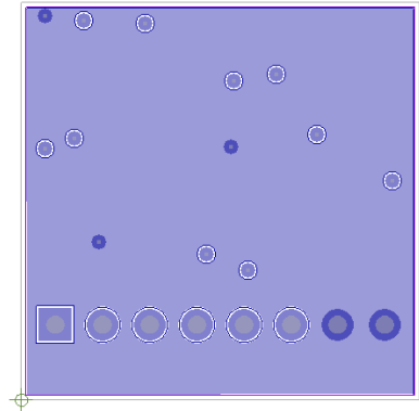
Figure 81. PCB Layout, Layer 2
