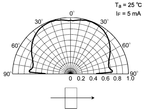
Fig. 8.8 Radiation Pattern
