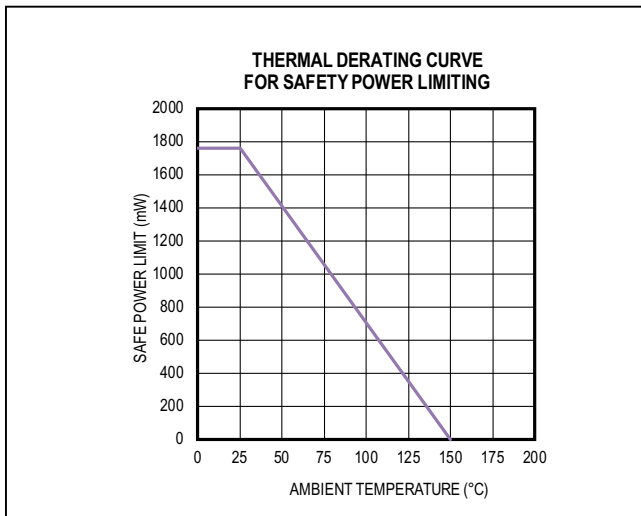
Figure 1. Thermal Derating Curve for Safety Power Limiting
