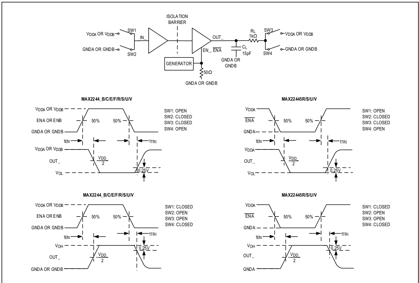
Figure 4. Enable to Output Timing ( t_{EN} , t_{TR} )
