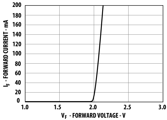
Figure 2. Forward Current vs. Forward Voltage, AS-AllnGaP.
