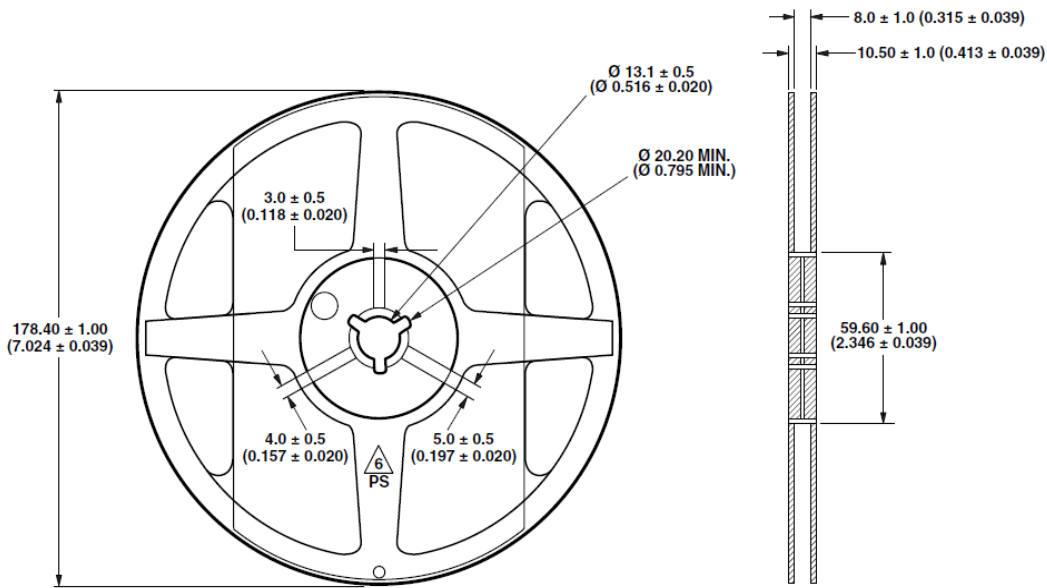
Figure 13: Reel Dimensions
