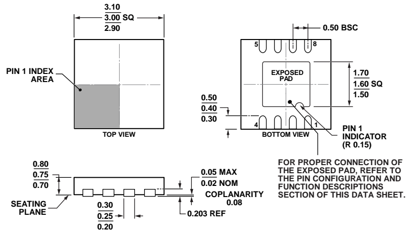
Figure 75. 8-Lead Lead Frame Chip Scale Package [LFCSO] 3 mm x 3 mm Body, Very Very Thin, Dual Lead (CP-8-12) Dimensions shown in millimeters
