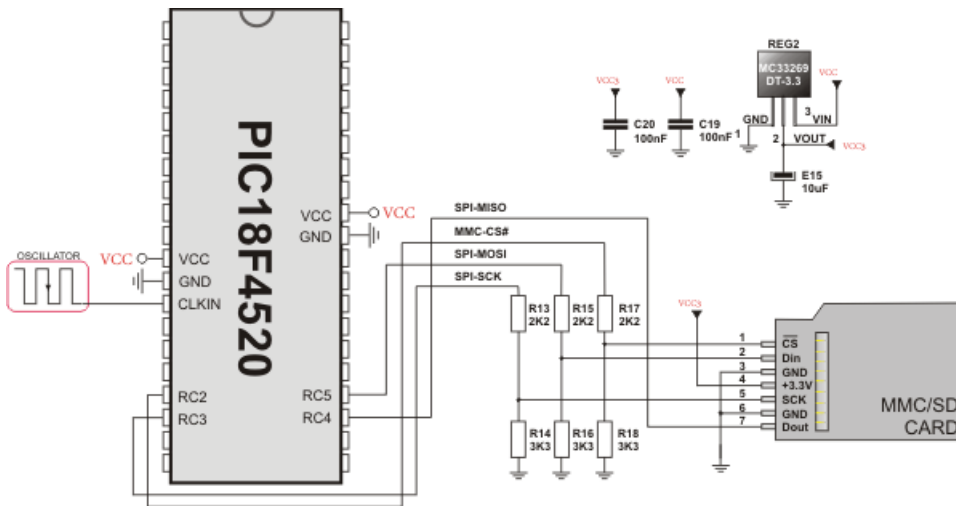
MMC interface
