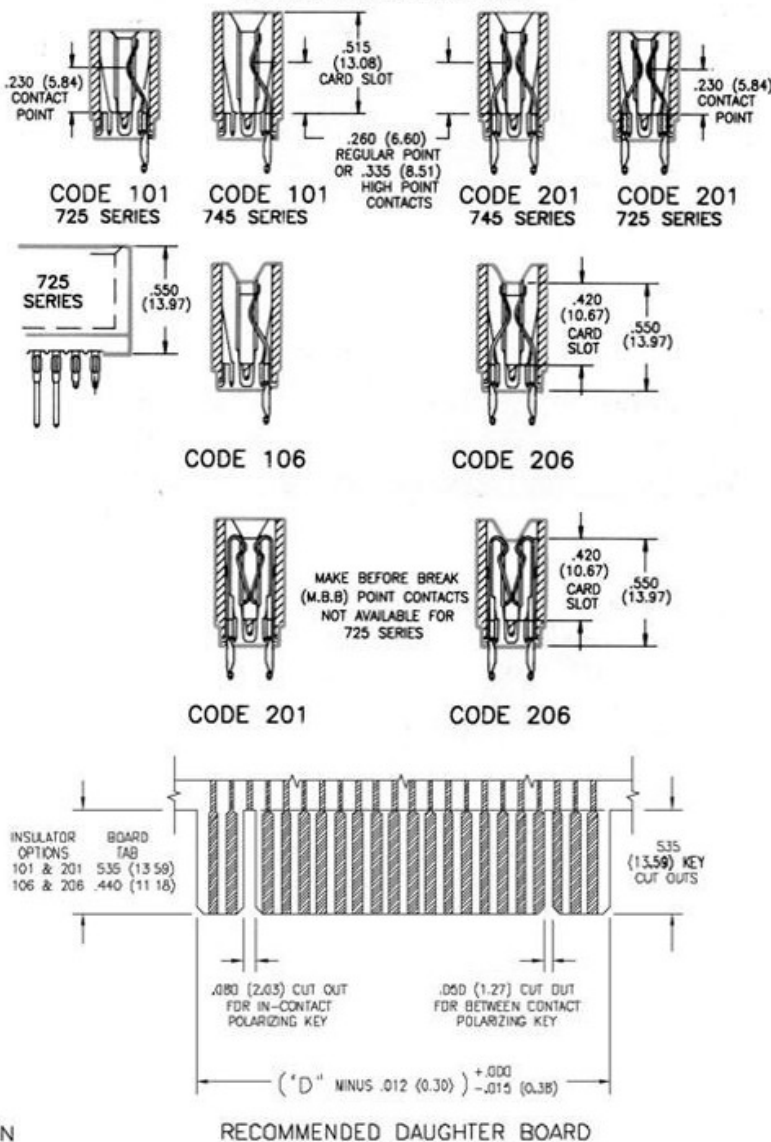
RECOMMENDED DAUGHTER BOARD
