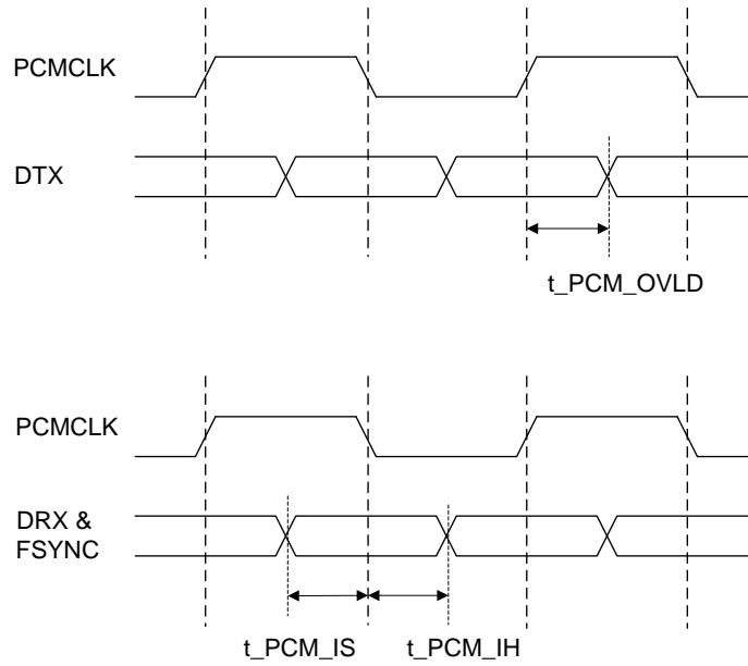
Figure 4-6 PCM Interface
