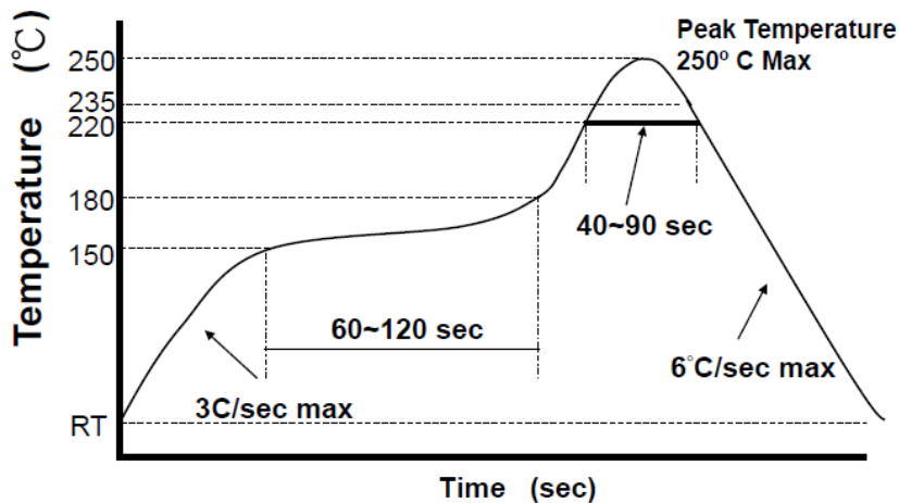
Figure 4-18 Reflow profile for MT7688
