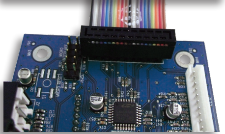
▲ DSP Interface Header connected to CRD-USBMASTER-DC-Z daughter card connected via JP1 ribbon cable enables real-time control of the DSP parameters shown in the DSP Composer .CPA signal flow file
