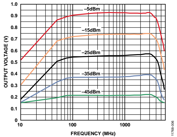
Figure 6. Typical V LOG vs. Frequency for Five RF Input Levels at 25°C
