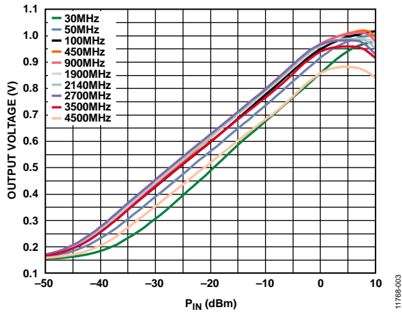
Figure 3. Typical V LOG vs. P IN over Frequency at 25°C
