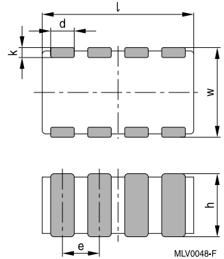
4-fold array
