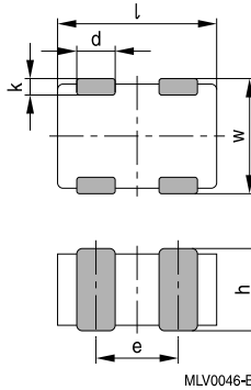
2-fold array
