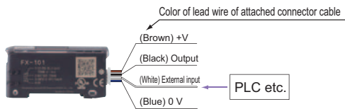
External input lines are equipped as standard
