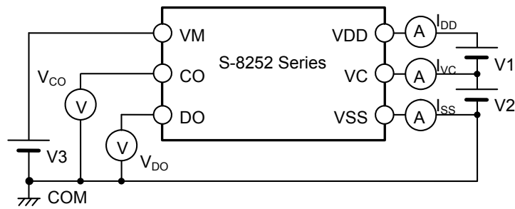
Figure 6 Test Circuit 2
