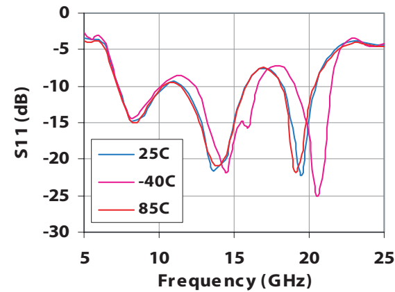
Figure 17b. Input Return Loss Over Temp
