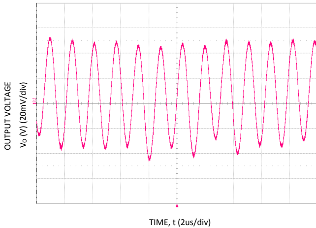
Figure 3. Typical output ripple and noise ( C_o=3 \times 10 \mu\text{F} + 470 \mu\text{F} , V_{IN} = 12\text{V} , I_o = I_{o,max} ).
