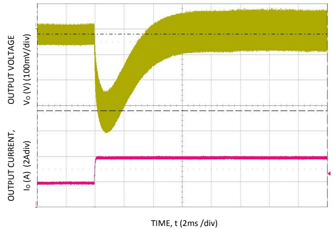
Figure 4. Transient Response to Dynamic Load Change from 50% to 100% at 12Vin, C_{out}=3 \times 10 \mu\text{F} + 470 \mu\text{F} , C_{Tune}=1000\text{pF} , R_{Tune}=30.1\text{k}\Omega
