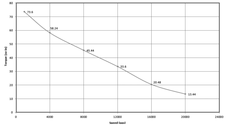
CUI P/N NEMA23-17-01PD-AMT112S Lin Engineering P/N WO-5718X-01P (1.8 Step Motor) 24 Vdc, 2.8 Amp/Phase, IB463, 1/2 Stepping
