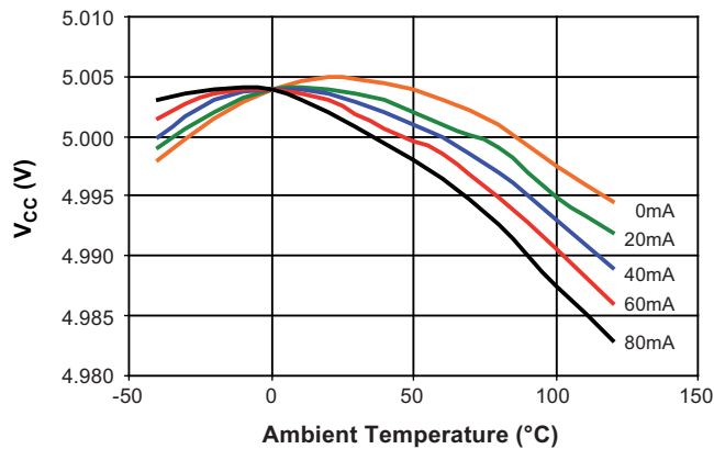
Figure 1-1. V_{CC} versus Temperature at Different Load Currents
