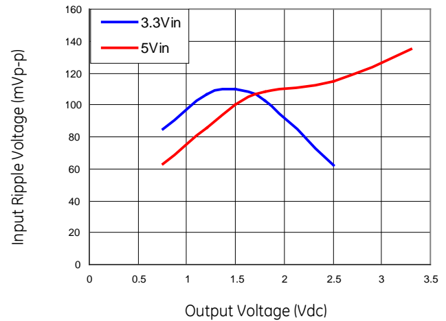
Figure 28. Input ripple voltage for various outputs with 1x22\mu F ceramic capacitor at the input (full-load).
