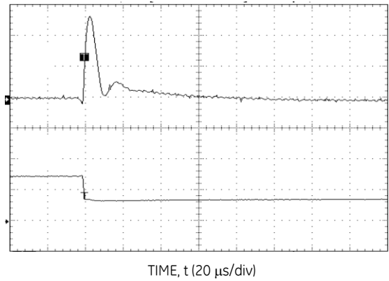
Figure 11. Transient Response to Dynamic Load Change from 100% to 50% of full load ( V_o = 3.3 Vdc).
