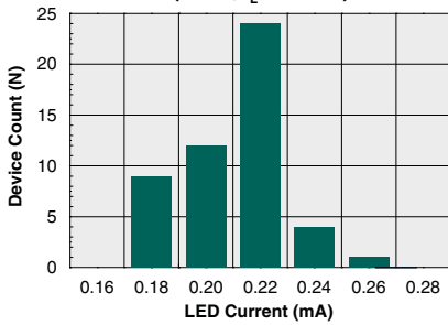
Typical I F for Switch Operation (N=50, I L =600mA)
