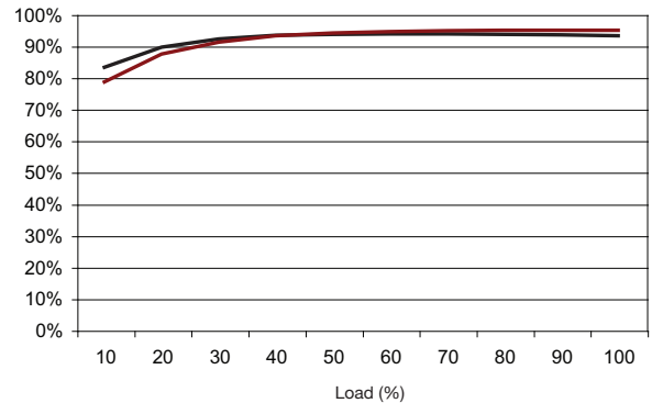
Figure 10 - AHM250PS48
