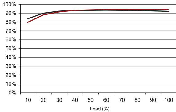
Figure 9 - AHM250PS24
