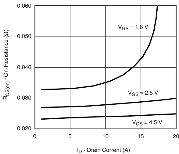
V_{GS} = 1.8\text{ V} V_{GS} = 2.5\text{ V} V_{GS} = 4.5\text{ V} On-Resistance vs. Drain Current and Gate Voltage
