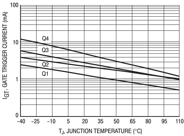
Figure 7. Typical Gate Trigger Current versus Junction Temperature
