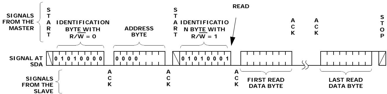
FIGURE 16. READ SEQUENCE
