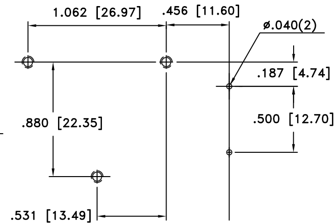
PCB LAYOUT
