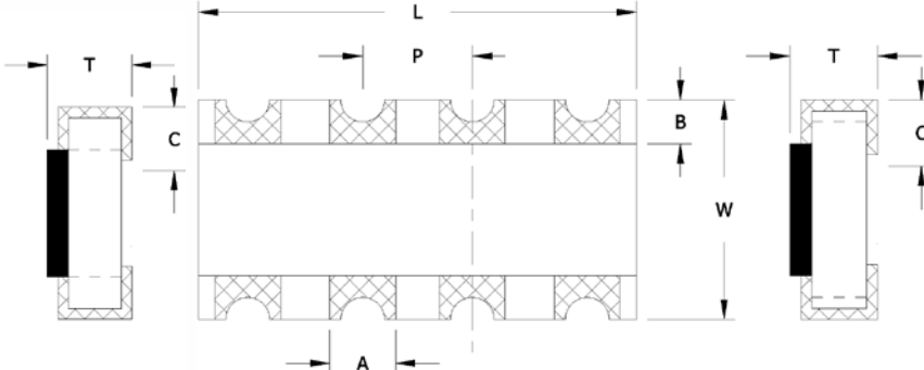
Package Drawing – Concave, Type X
