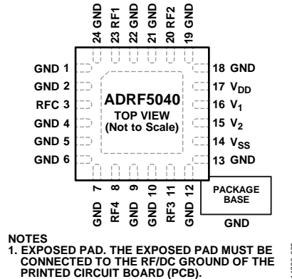
Figure 5. Pin Configuration
