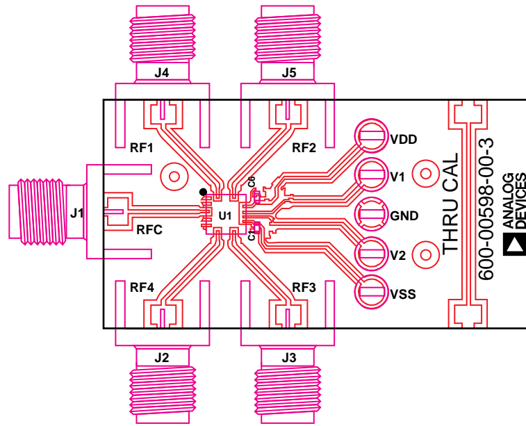
Figure 27. Evaluation PCB
