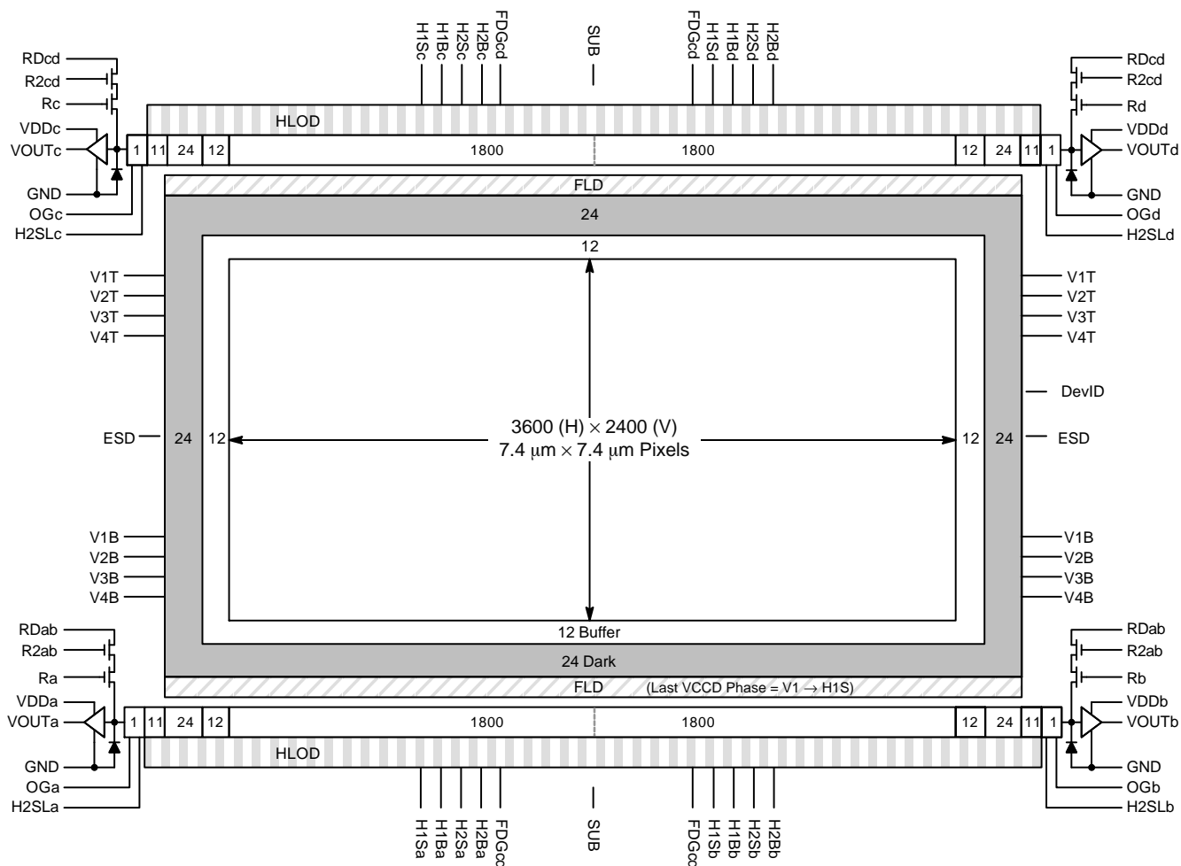
Figure 2. Block Diagram
