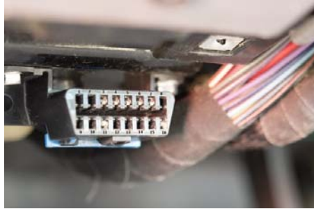
Data Link Connector in a 1998 Jeep Cherokee, with the pins labeled.
