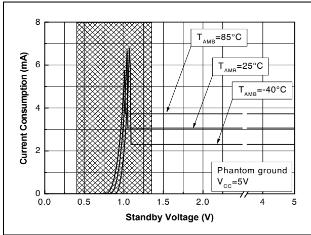
Figure 74. Current consumption vs. standby voltage, V CC = 5 V, PHG
