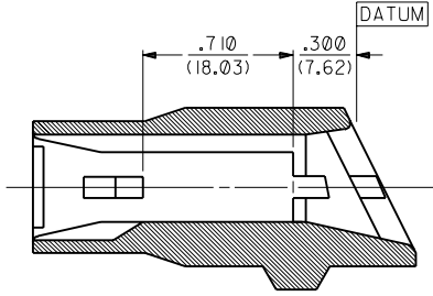
SECTION A-A TYPICAL CORE
