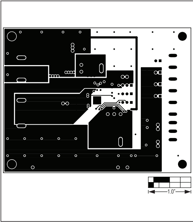
Figure 5. MAX16920B EV Kit PCB Layout—Inner Layer 3
