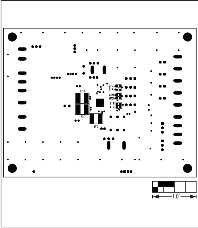
Figure 7. MAX16920B EV Kit Component Placement Guide—Solder Side
