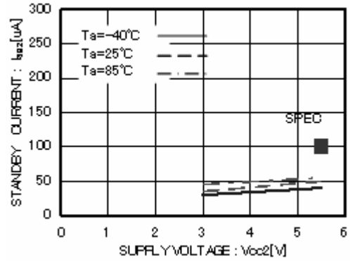
Figure 23. Standby Current2 I_{SB2}
