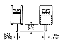
08 Printed Circuit
