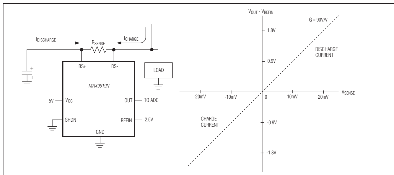
Figure 2. Bidirectional Operation
