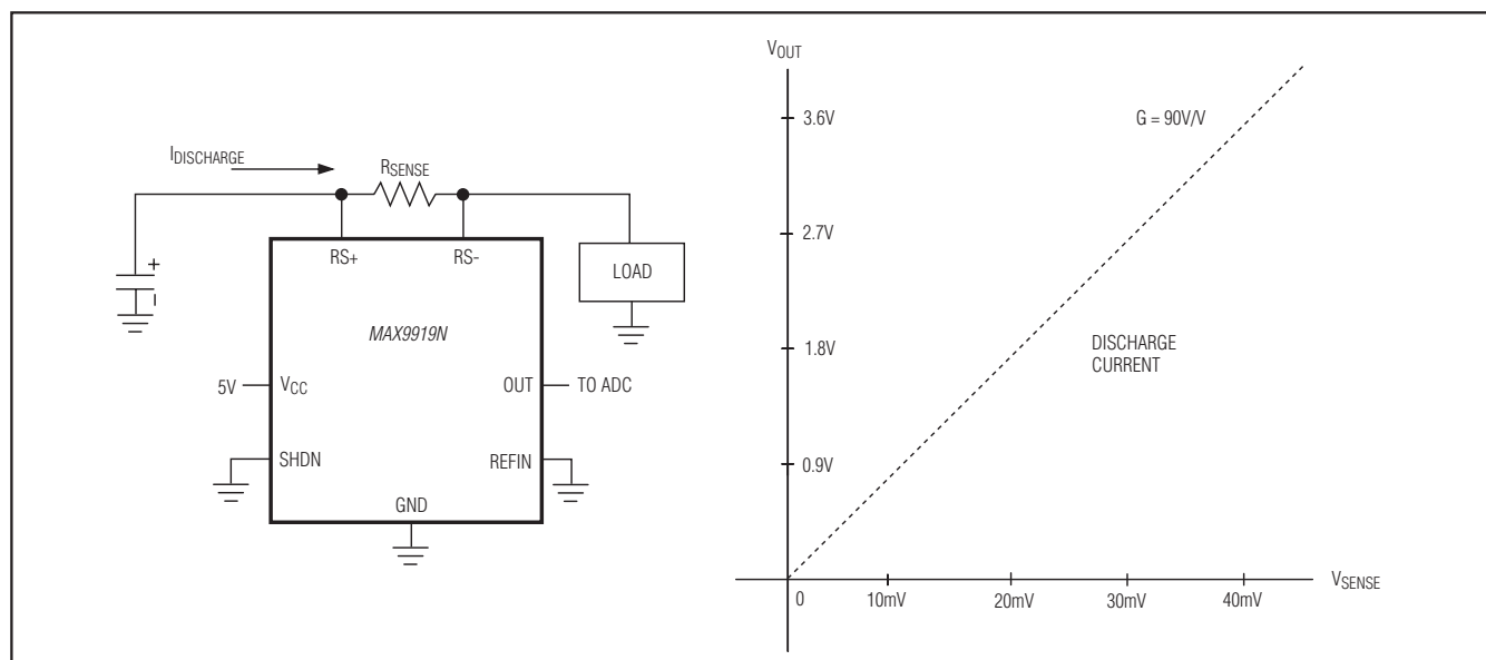
Figure 1. Unidirectional Operation
