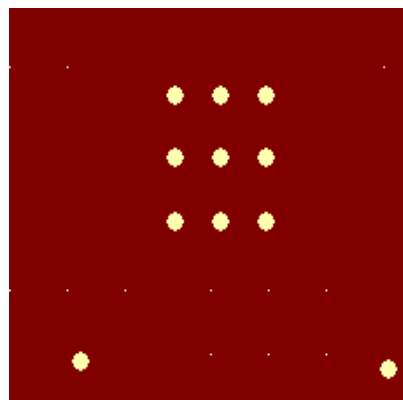
INTERNAL GROUND PLANE (24 LD QFN)
