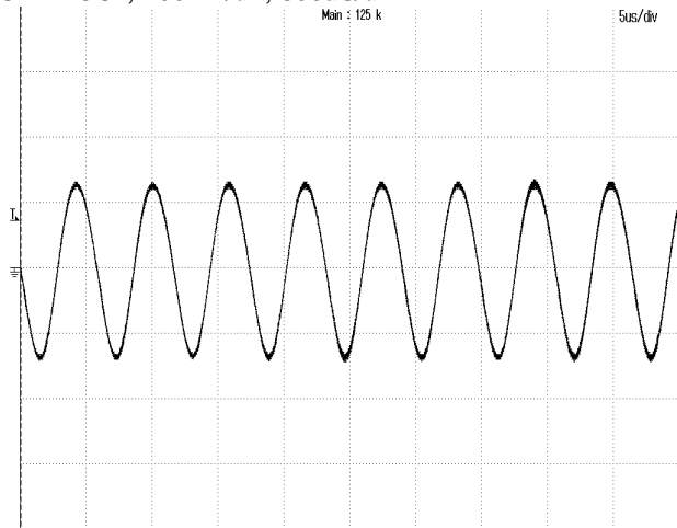
Figure 7: Output ripple & noise at 48Vin, 24A lout CH1:VOUT, 50mV/div, 5µS/div
