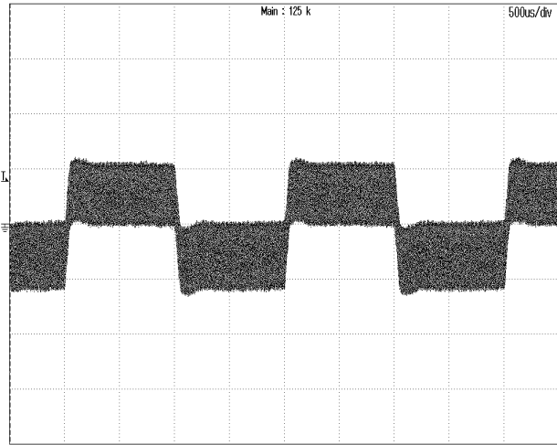
Figure 5: Dynamic response to load step 12A~18A with 0.1A/µS slew rate at 48Vin CH1:VOUT, 100mV/div, 500µS/div
