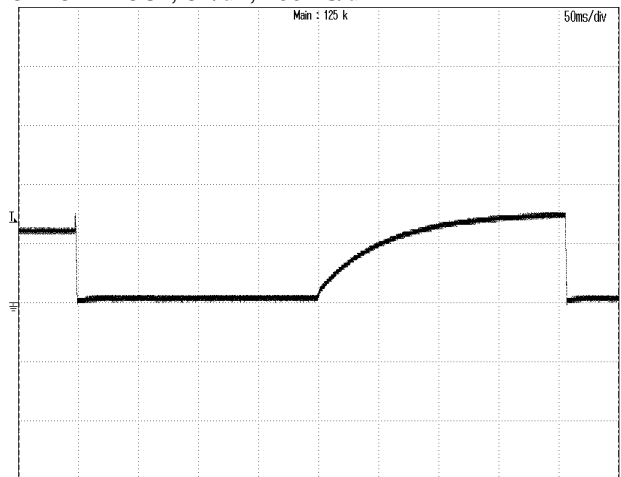
Figure 8: Output over voltage protection at 48Vin, 24A lout CH1:VOUT, 10V/div, 50mS/div
