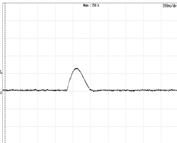
Figure 15: Inrush current @ Vin=48V CH1:lin, 2A/div, 200nS/div Max current 2.7A, I2t=1.24E-7 A 2 S
